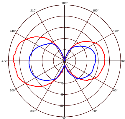
Photometric Diagram
